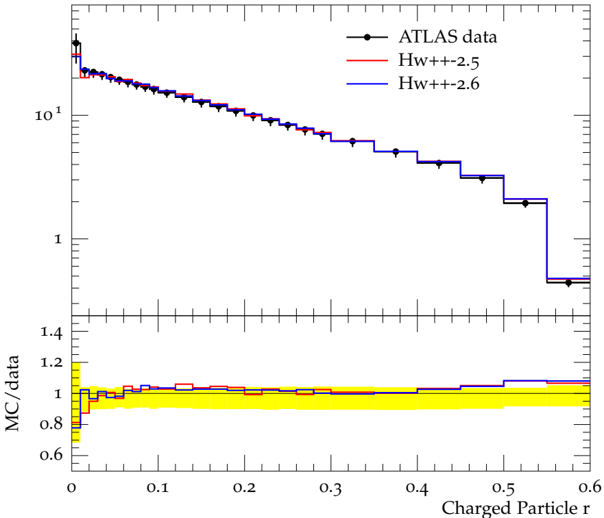
Charged jet \rho_{\text{ch}}(r) (anti- k_t , R = 0.6 , y 0.5-1.0, p_{\perp} 6.0-10.0)
