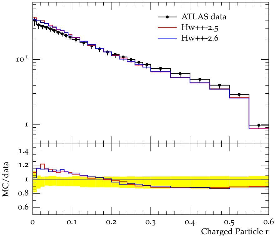
Charged jet \rho_{\text{ch}}(r) (anti- k_t , R = 0.6 , y 0.5-1.0, p_{\perp} 10.0-15.0)
