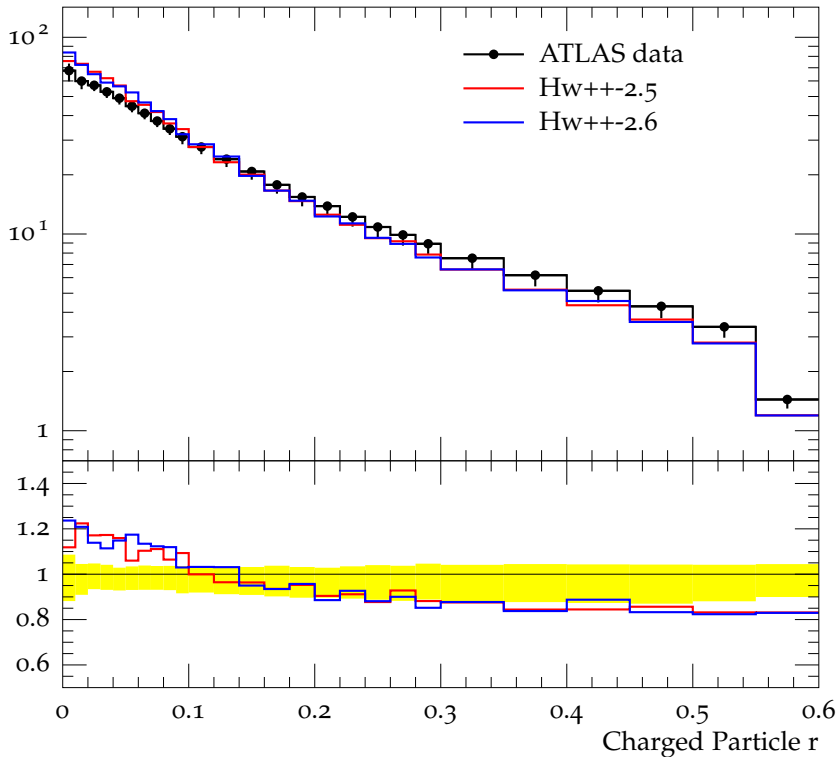
Charged jet \rho_{\text{ch}}(r) (anti- k_t , R = 0.6 , y 0.5-1.0, p_{\perp} 15.0-24.0)
