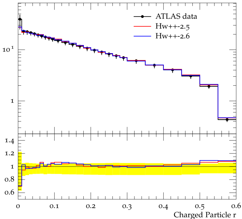
Charged jet \rho_{\text{ch}}(r) (anti- k_t , R = 0.6 , y 1.0-1.5, p_{\perp} 6.0-10.0)
