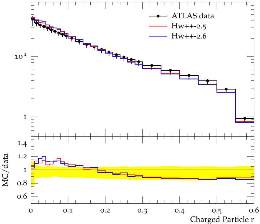
Charged jet \rho_{\text{ch}}(r) (anti- k_t , R = 0.6 , y 1.0-1.5, p_{\perp} 10.0-15.0)
