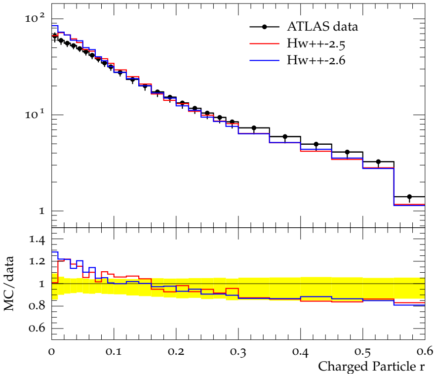
Charged jet \rho_{\text{ch}}(r) (anti- k_t , R = 0.6 , y 1.0-1.5, p_{\perp} 15.0-24.0)
