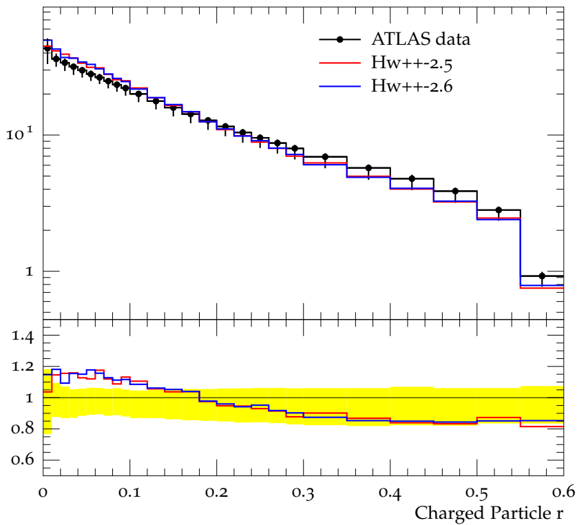
Charged jet \rho_{\text{ch}}(r) (anti- k_t , R = 0.6 , y 1.5-1.9, p_{\perp} 10.0-15.0)
