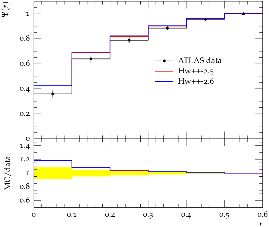
Jet shape \Psi for p_{\perp} \in 30\text{--}40\text{ GeV} , y \in 2.1\text{--}2.8
