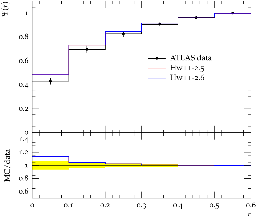
Jet shape \Psi for p_{\perp} \in 40\text{--}60\text{ GeV} , y \in 1.2\text{--}2.1
