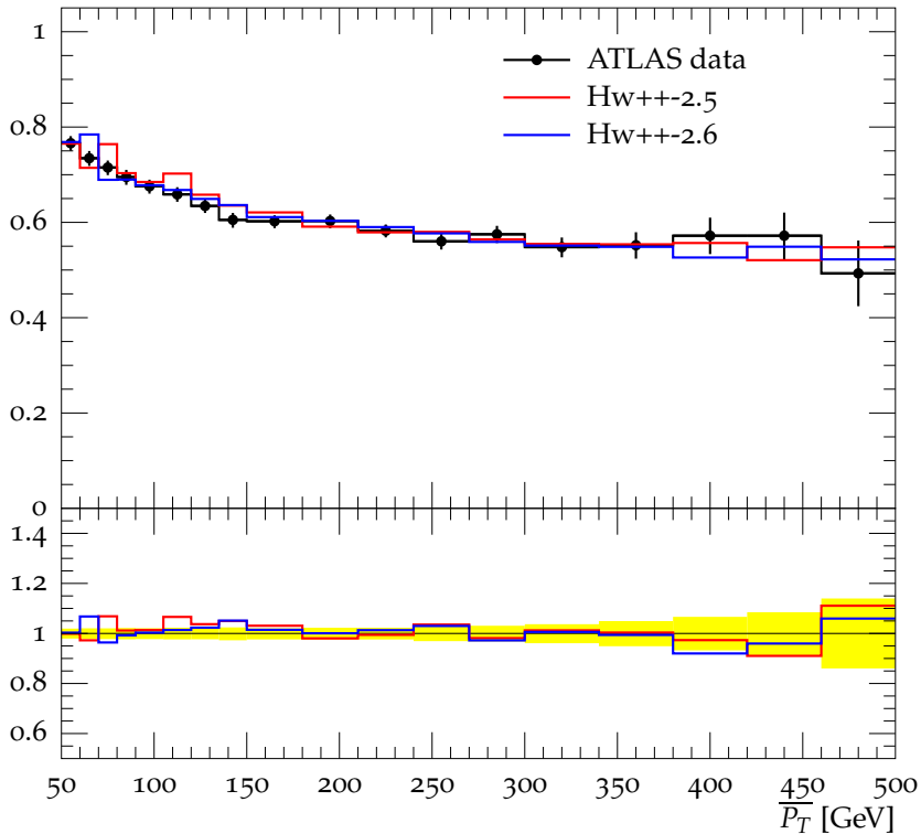
Gap fraction vs \overline{P_T} for 1.0 < |\Delta y| < 2.0 , Fwd/Bwd
