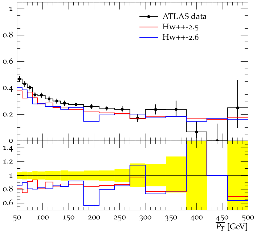
Gap fraction vs \overline{P_T} for 3.0 < |\Delta y| < 4.0 , Fwd/Bwd
