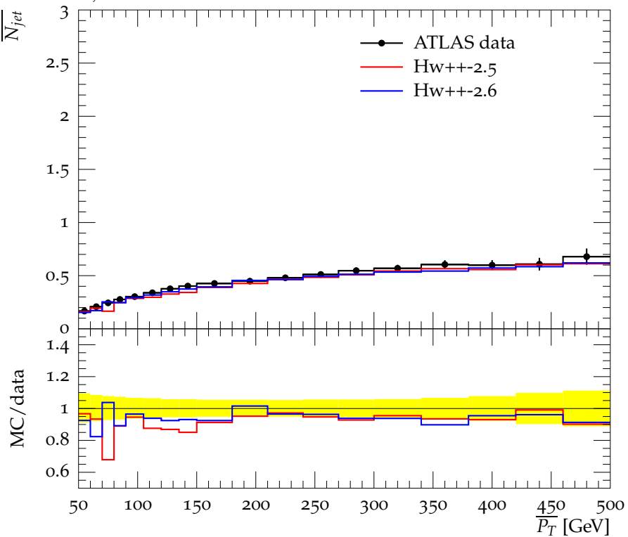
\overline{N}_{jet} vs \overline{P}_T for 1 < |\Delta y| < 2 , Leading Jet
