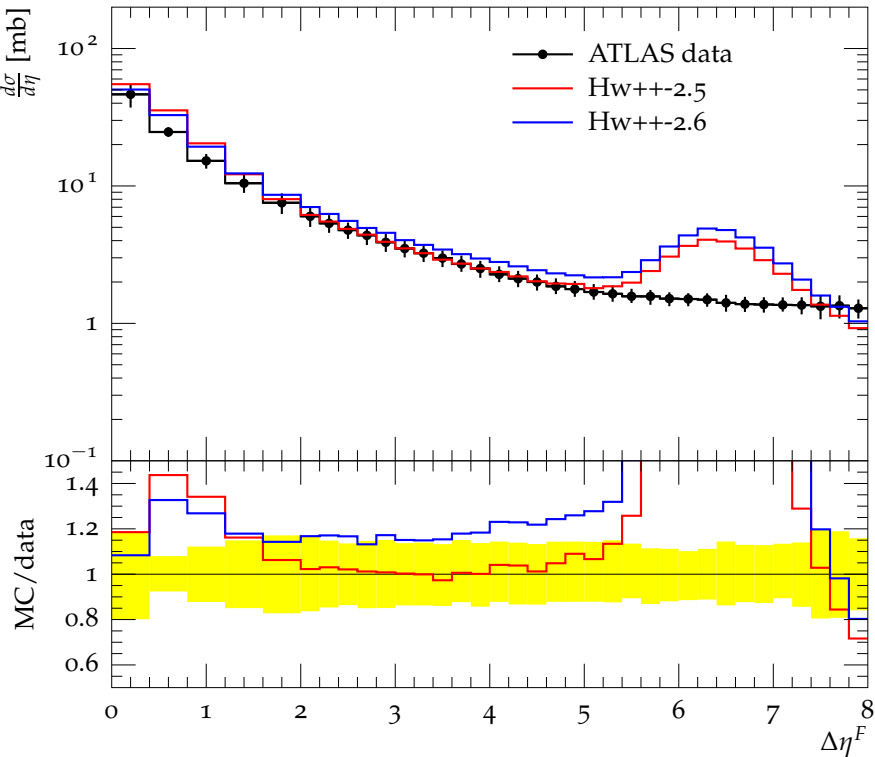
Rapidity gap size in \eta starting from \eta = \pm 4.9 , p_T > 600 MeV
