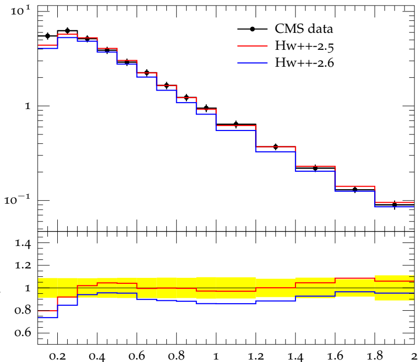
Charged hadron p_{\perp} for |\eta| = 0.1 at \sqrt{s} = 0.9 TeV
