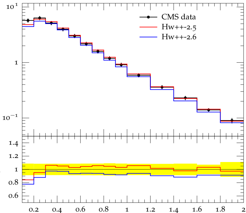
Charged hadron p_{\perp} for |\eta| = 0.7 at \sqrt{s} = 0.9 TeV
