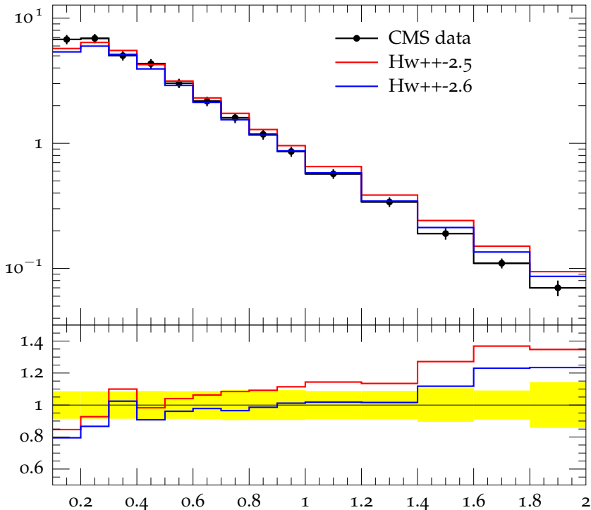
Charged hadron p_{\perp} for |\eta| = 2.1 at \sqrt{s} = 0.9 TeV
