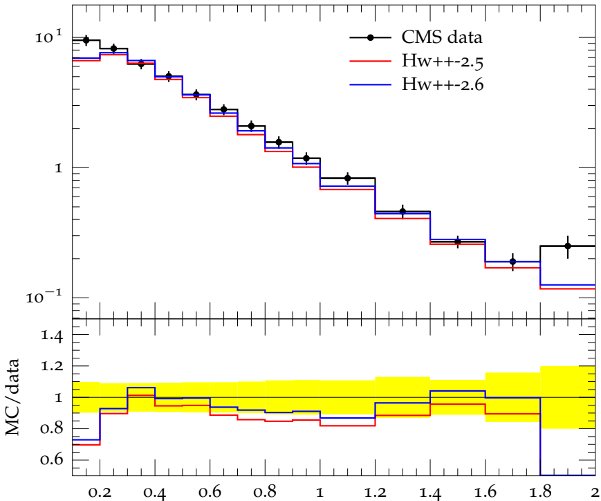
Charged hadron p_{\perp} for |\eta| = 2.3 at \sqrt{s} = 2.36 TeV
