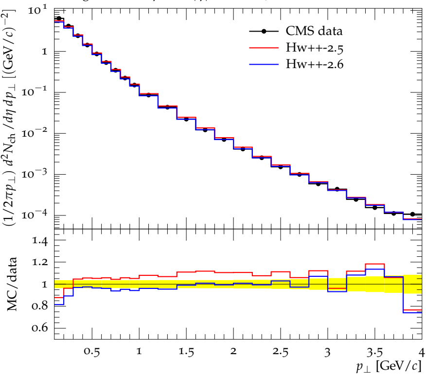
Charged hadron p_{\perp} for |\eta| < 2.4 at \sqrt{s} = 0.9 TeV
