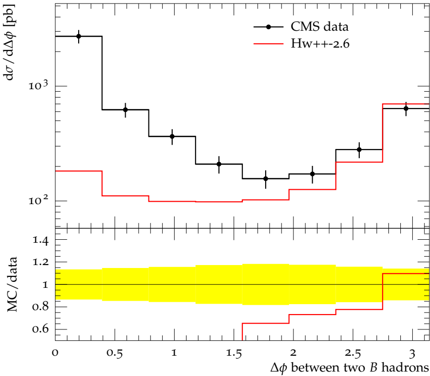
B\bar{B} production cross-section (leading jet p_{\perp} > 120 GeV)
