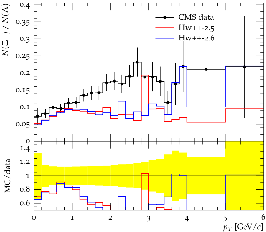
\Xi^- / \Lambda versus transverse momentum at \sqrt{s} = 0.9 TeV
