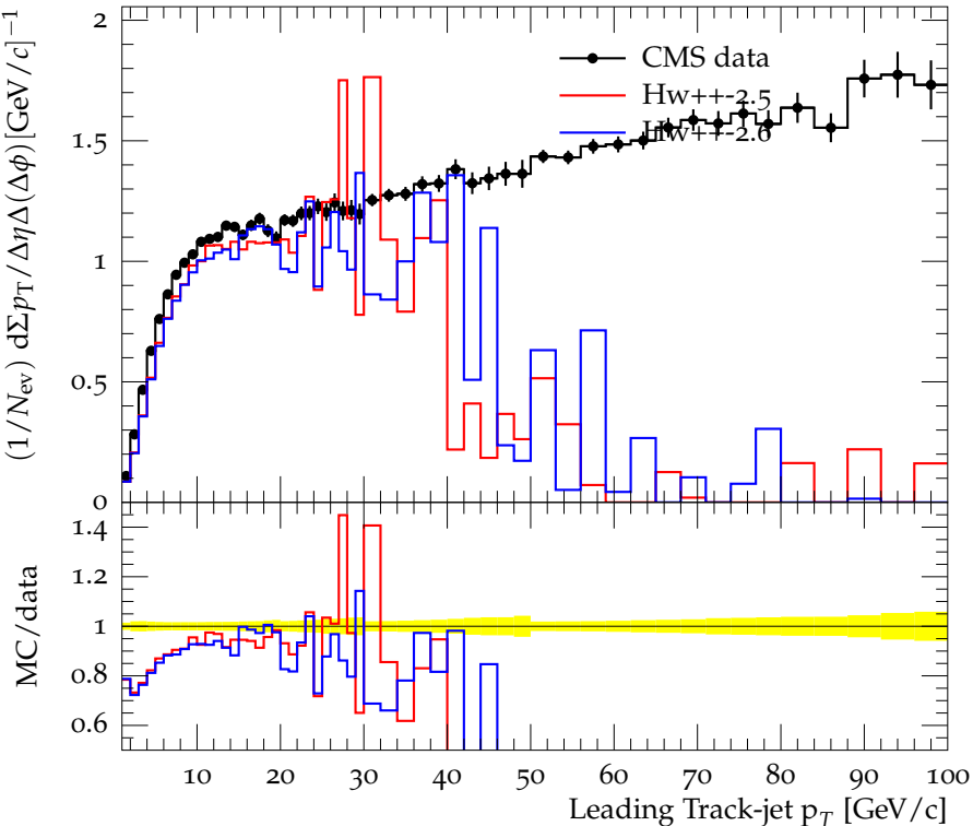
Profile \Sigma p_T at \sqrt{s} = 7 TeV, 60 < |\Delta\phi| < 120
