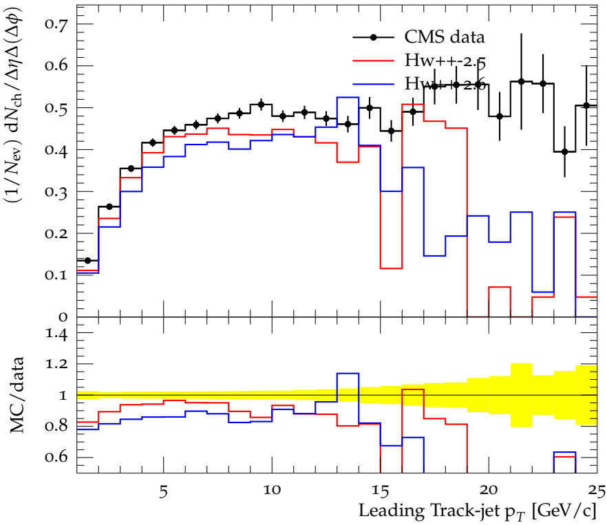
Profile N_{\text{ch}} at \sqrt{s} = 0.9 TeV, 60 < |\Delta\phi| < 120
