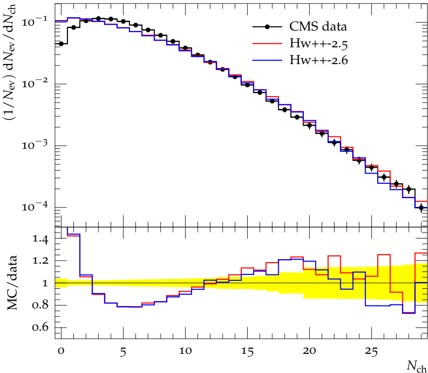
Distribution N_{\text{ch}} at 7 TeV, \max p_{\text{T}} > 20 \text{ GeV}/c
