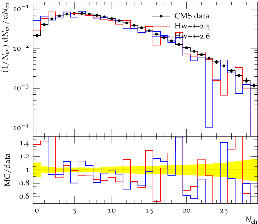
Distribution N_{\text{ch}} at 7 TeV, \max p_{\text{T}} > 3 \text{ GeV}/c
