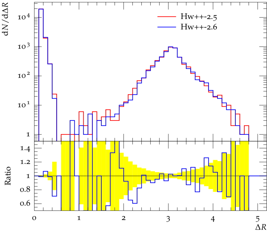
\Delta R between leading jet and leading photon
