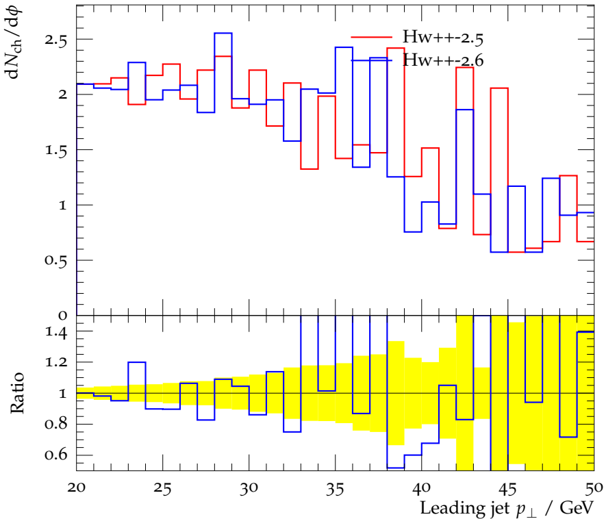
TransMIN region charged particle density
