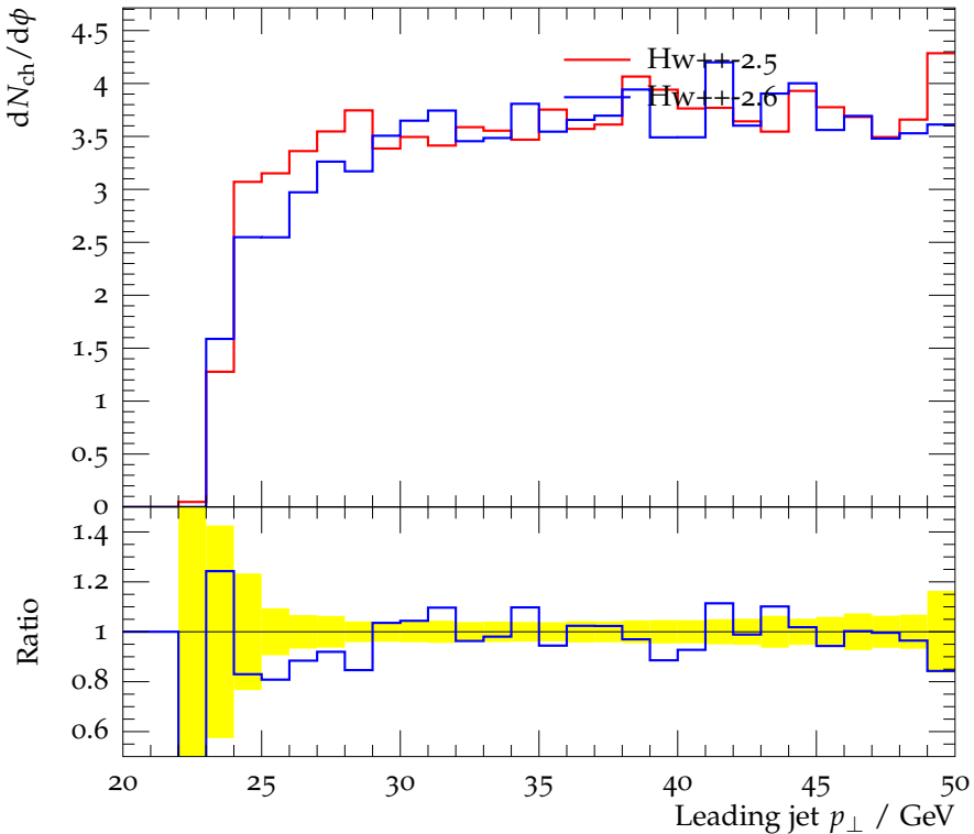
Transverse region charged particle density
