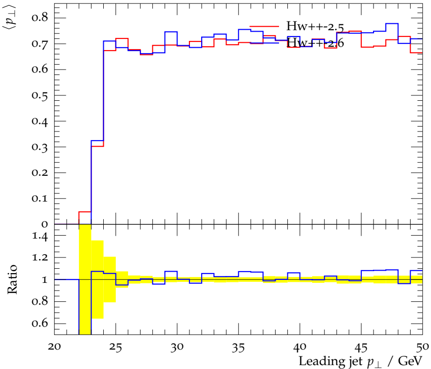
Transverse region charged pT average
