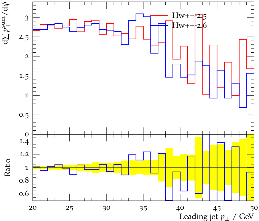
Transverse region charged pT sum density
