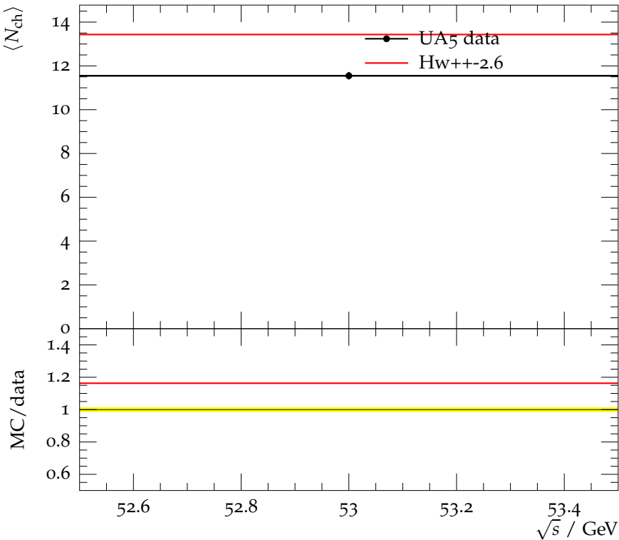
Mean charged multiplicity for pp collisions at \sqrt{s} = 53 GeV
