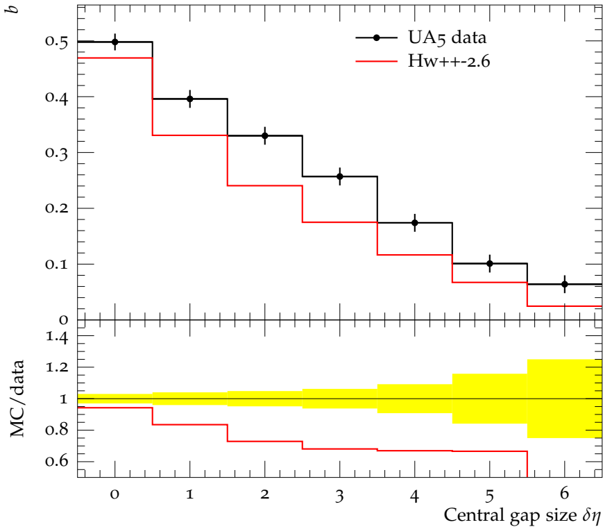
Forward-backward correlation b vs. gap size \sqrt{s} = 200
