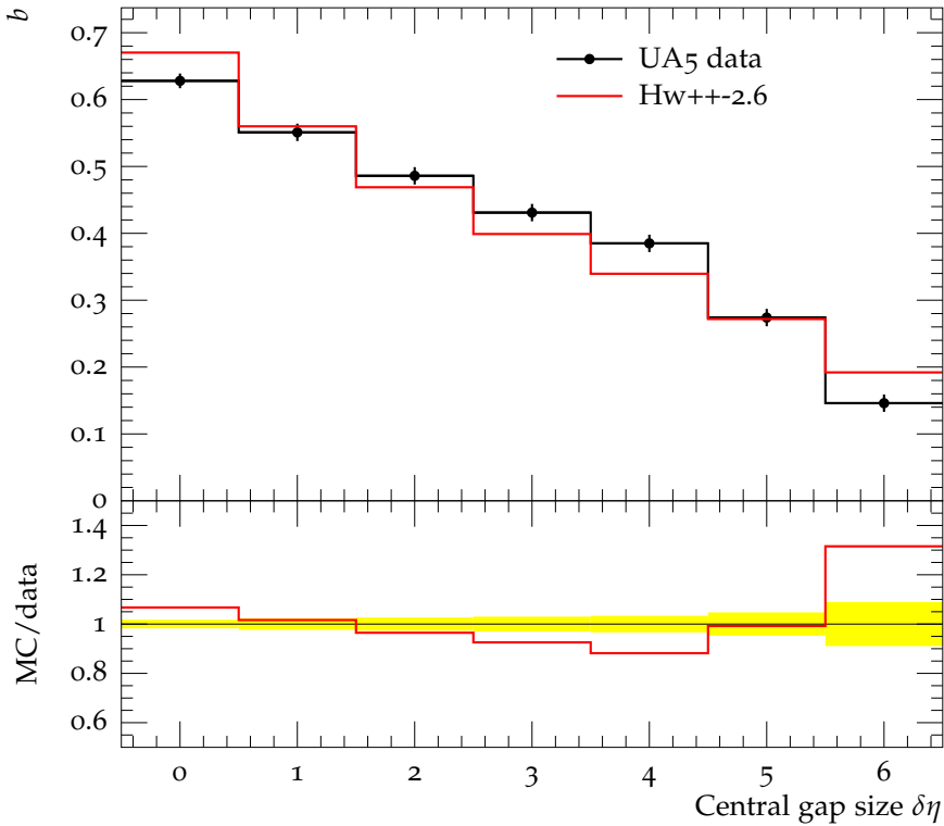
Forward-backward correlation b vs. gap size \sqrt{s} = 900
