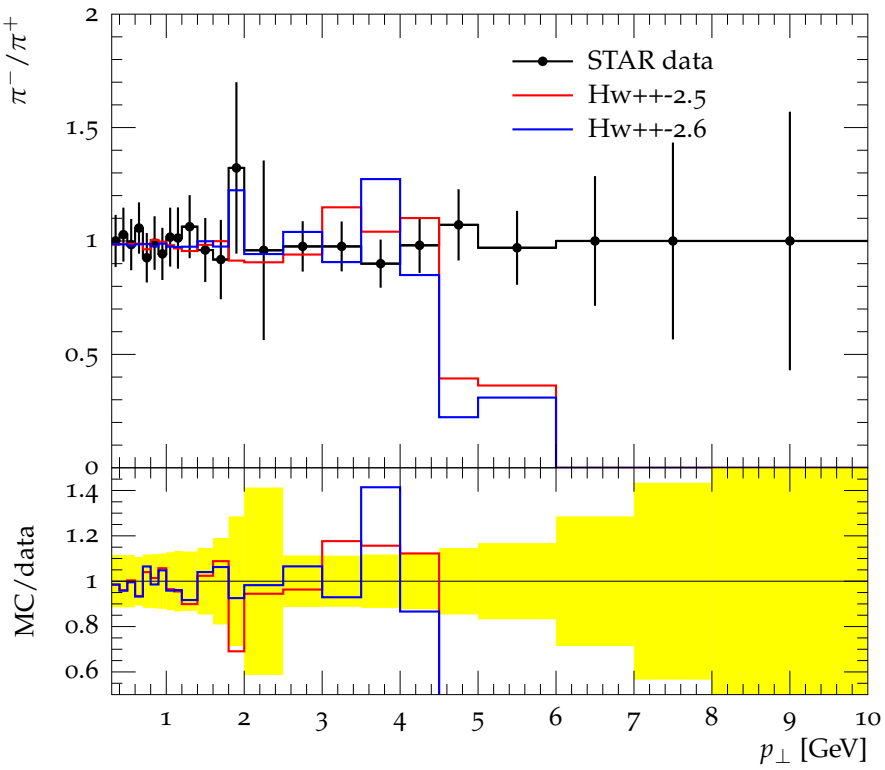
Ratio of \pi^-/\pi^+ as function of p_\perp
