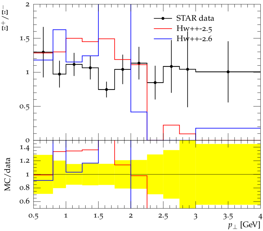
Ratio of \Xi^+/\Xi^- as function of p_\perp
