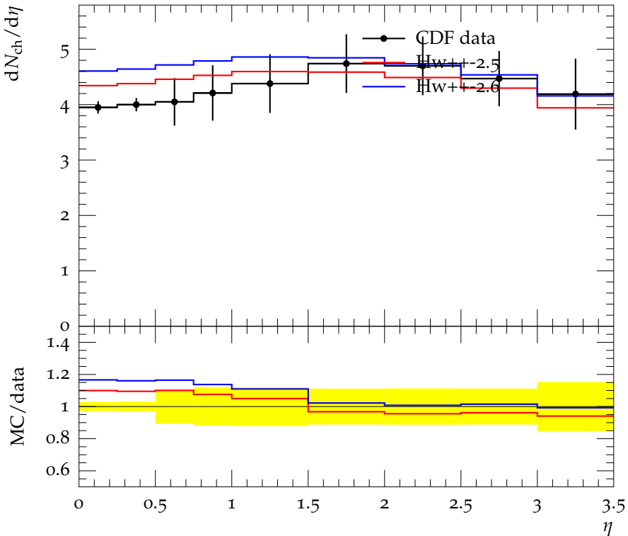
Pseudorapidity distribution at \sqrt{s} = 1800 GeV
