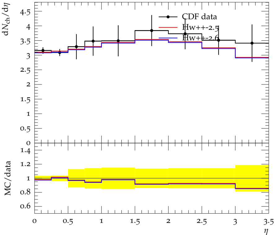
Pseudorapidity distribution at \sqrt{s} = 630 GeV
