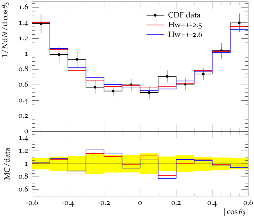
Leading jet angle in inclusive 3-jet events
