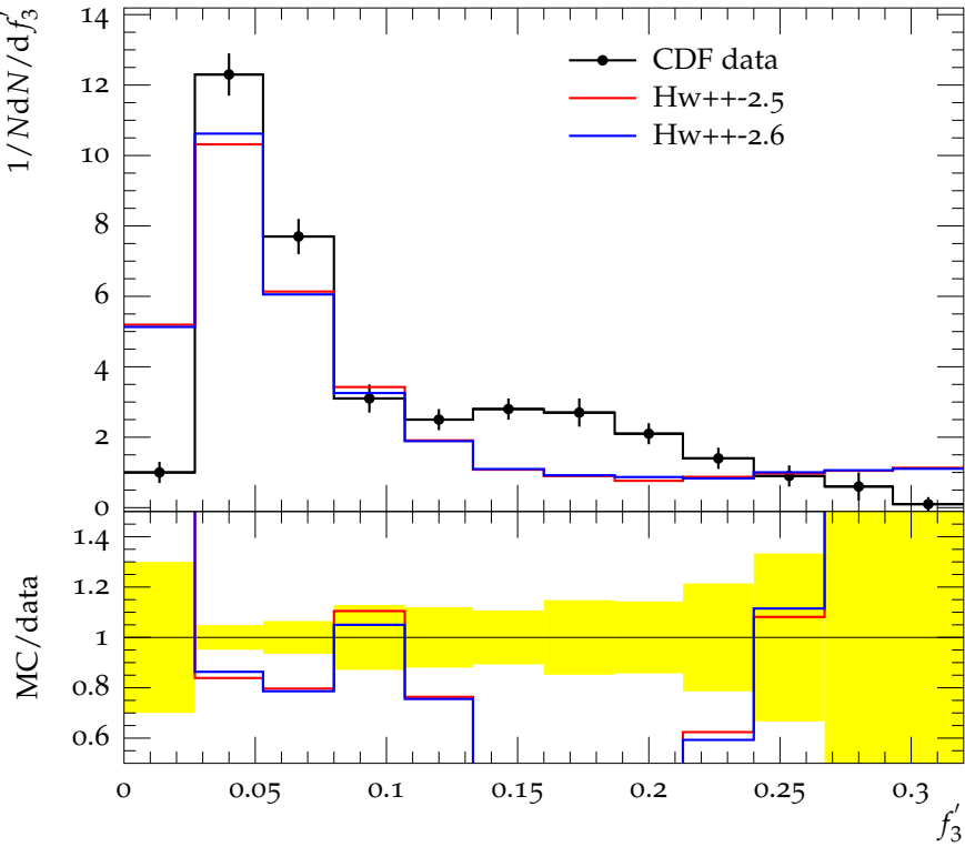
Single-jet mass fraction in inclusive 4-jet events
