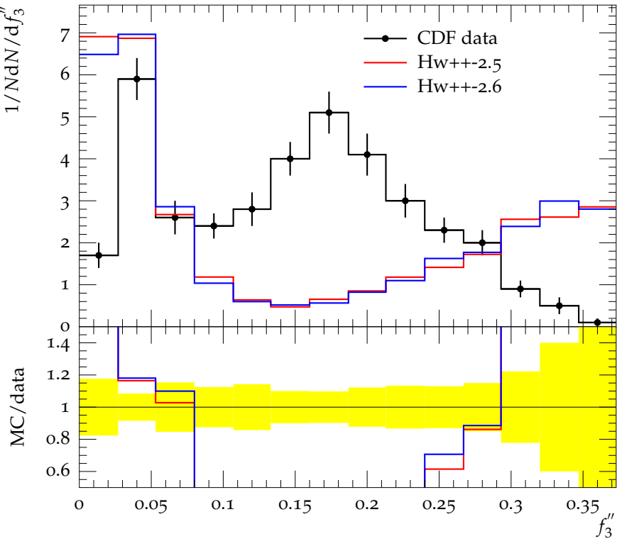
Single-jet mass fraction in inclusive 5-jet events
