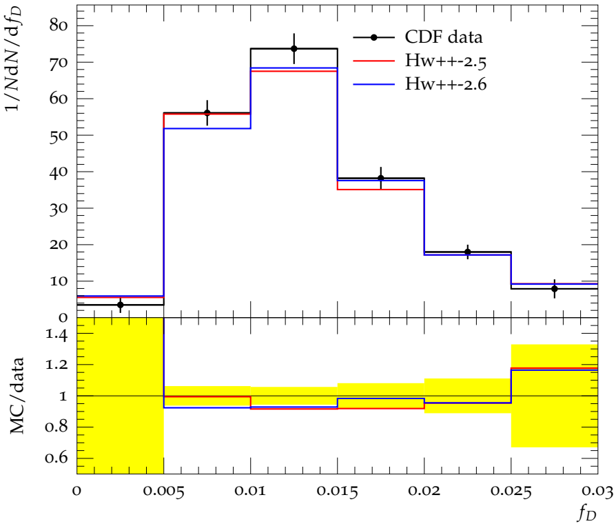
Single-body mass fraction in inclusive 5-jet events
