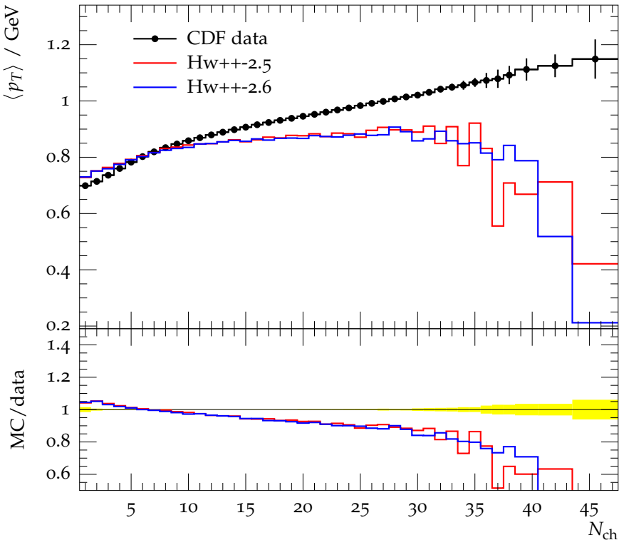
Mean track p_T vs multiplicity, |\eta| < 1 , p_{\perp} > 0.4 GeV
