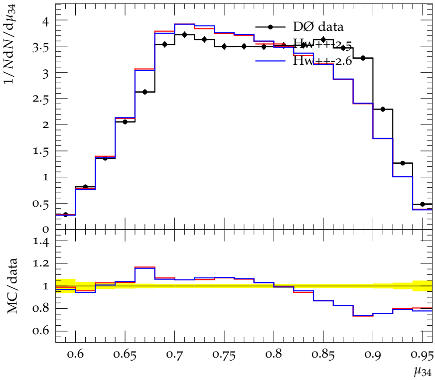
Scaled invariant mass of jet pair
