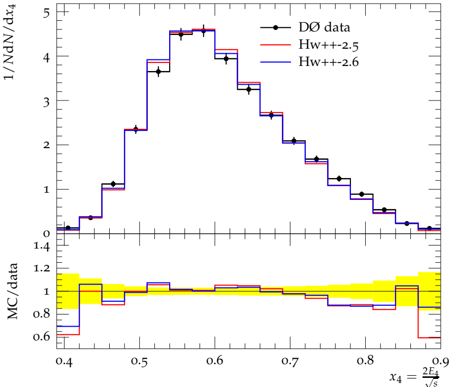
Energy fraction of 2nd jet in 4-jet events
