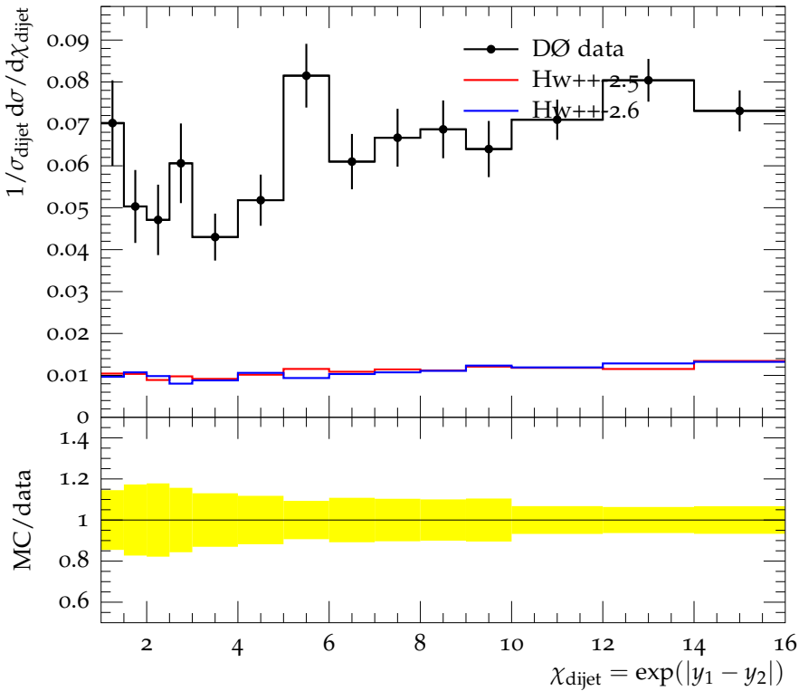
Dijet angular distribution in 0.25 < M_{jj}/\text{TeV} < 0.3
