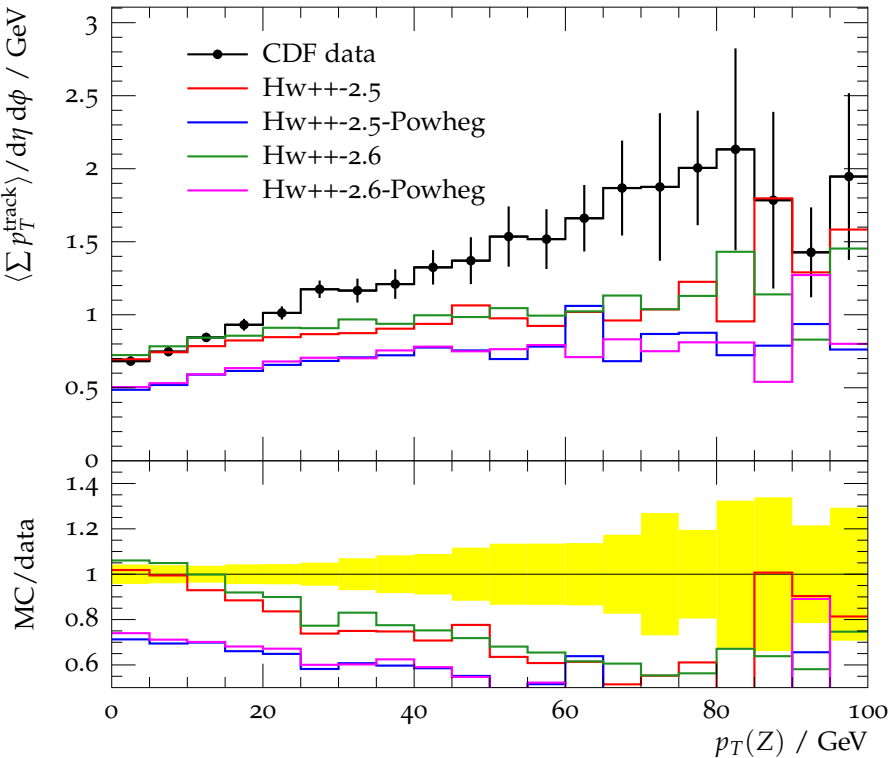
TransMAX region charged p_{\perp}^{\text{sum}} density
