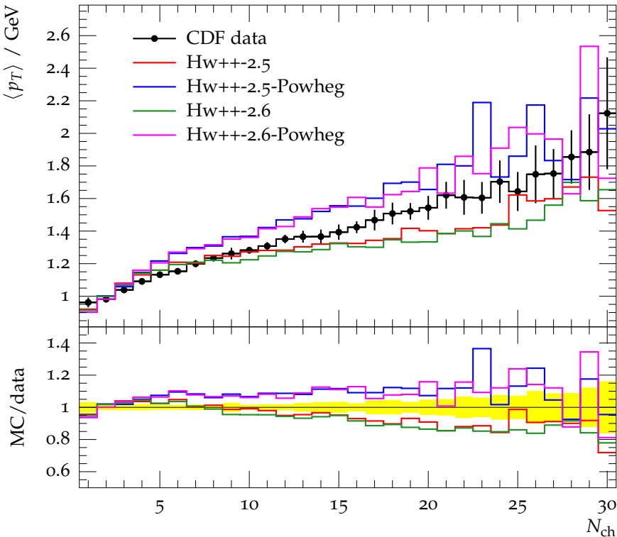
Average charged p_{\perp} vs charged multiplicity
