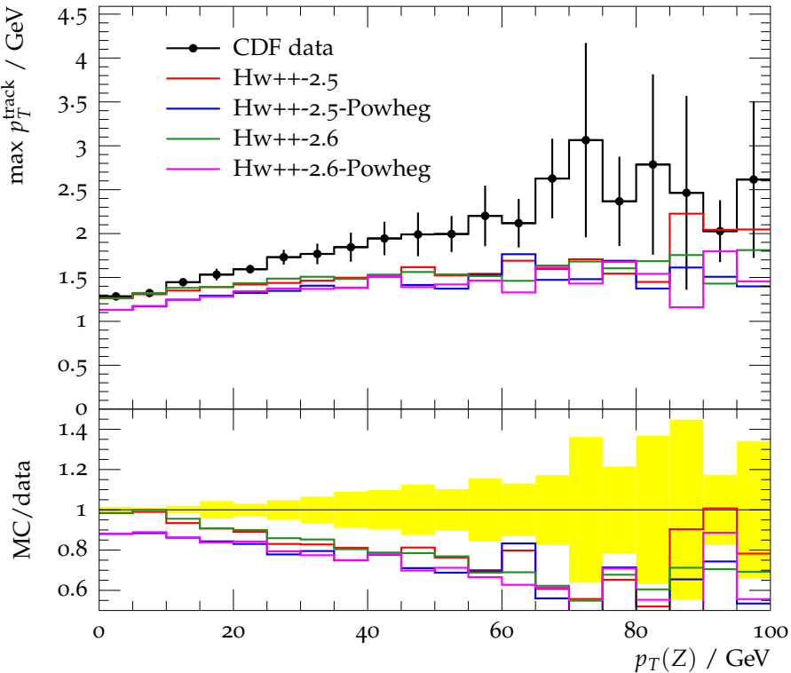
Transverse region charged p_{\perp} maximum
