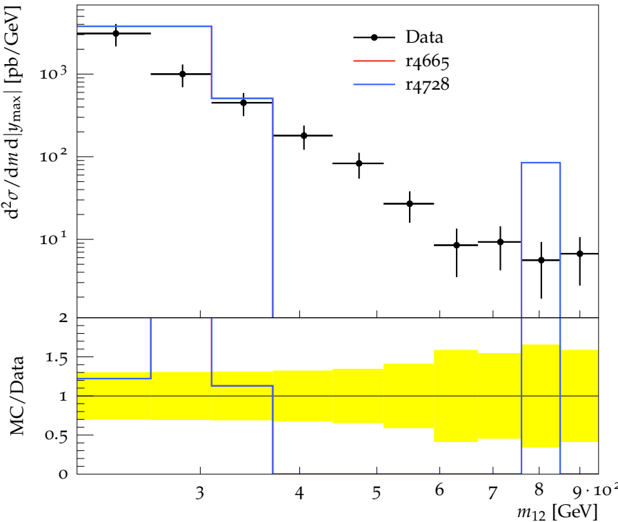
Dijet mass spectrum for 0.8 < |y_{\max}| < 1.2 . anti-KT, R = 0.6 .
