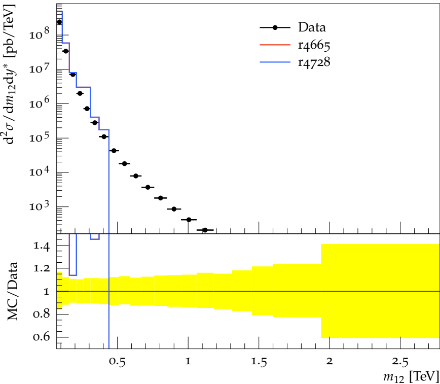
Dijet double-diff. x-section, anti- k_t 0.4 ( y^* < 0.5 )
