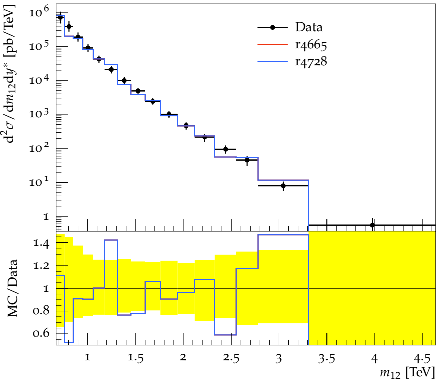
Dijet double-diff. x-section, anti- k_t 0.4 ( 2.5 \leq y^* < 3.0 )
